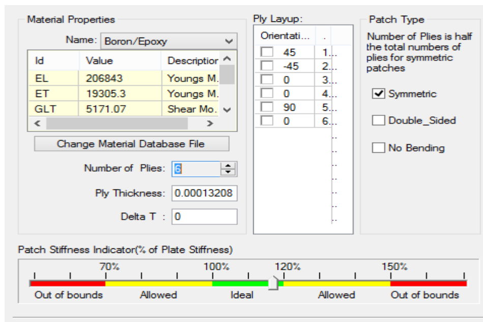
Figure III.6: Interface du composite Bore/Epoxy.
