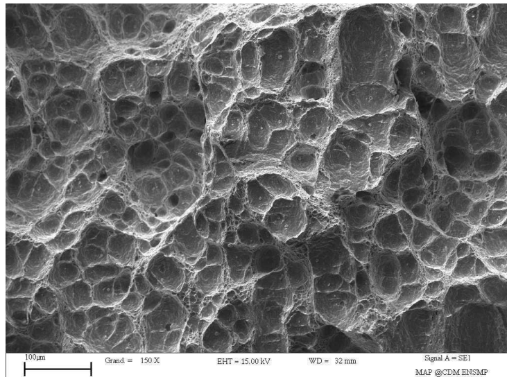
Figure I.10.: Rupture ductile aciers X100
