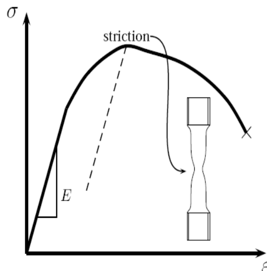
Figure I.9: Matériaux ductiles
