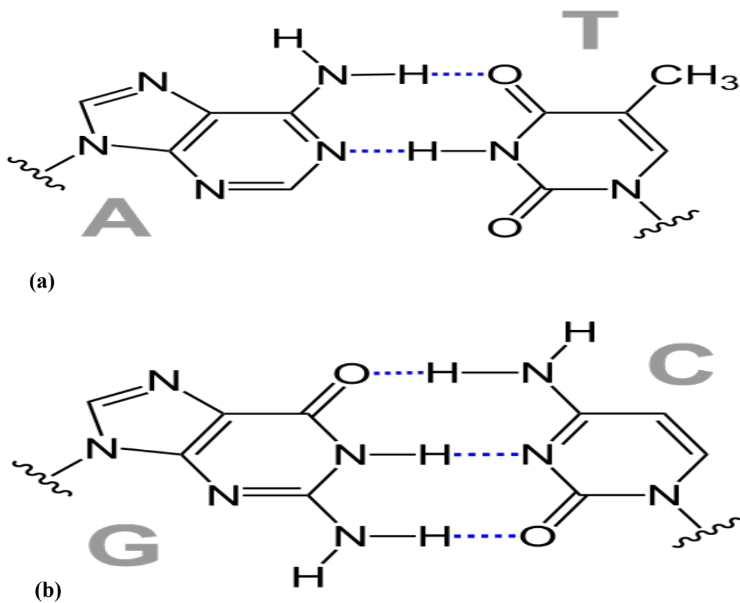
Figure 3. Structure of Purine and Pyrimidine Bases
