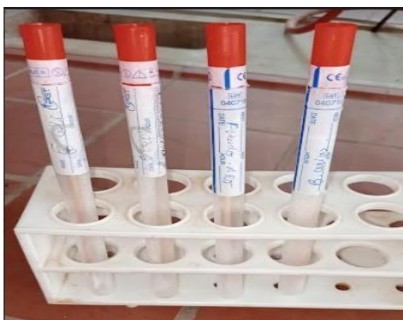
Figure II.22: Bacterial strains.
