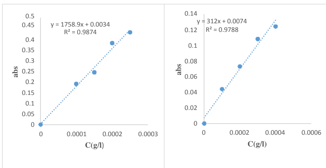
Figure 3: The calibration line of Chamomile.
