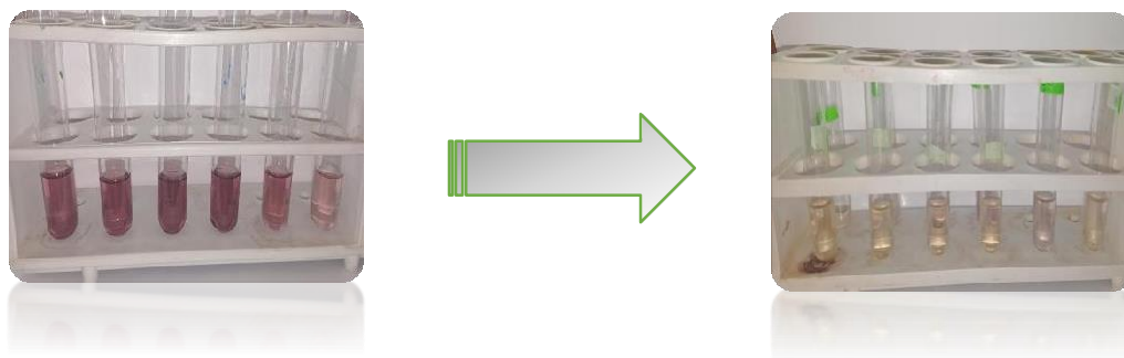
Figure II.30: Antioxidant activity protocol.
