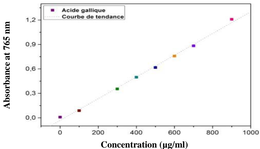
Figure 5 : Gallic acid calibration curve.
