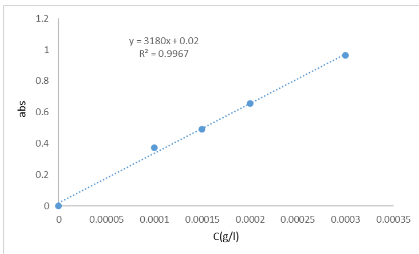
Figure II.21: The calibration line of Thymeleae.
