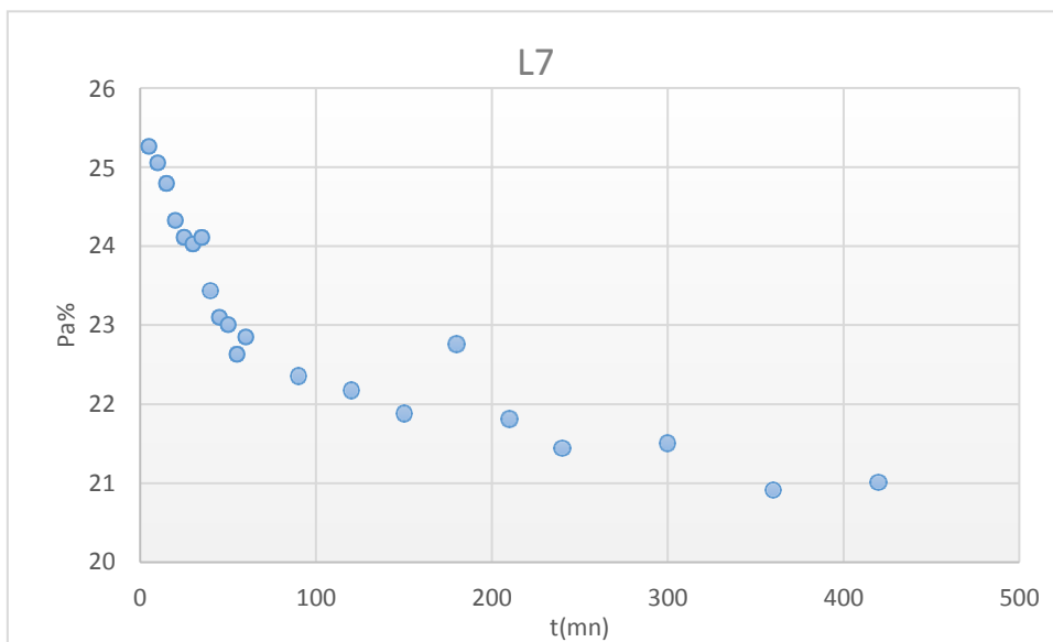
Figure III.15: Liberation curve of Thy from L7.
