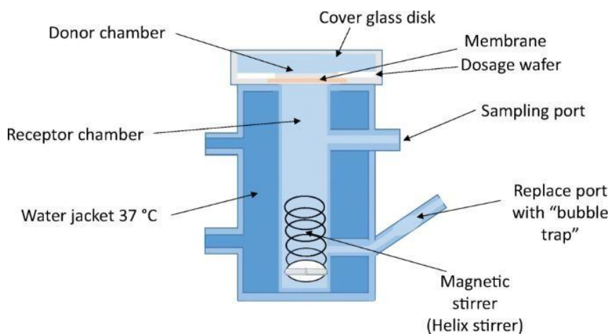
Figure II.18: Franz cell.
