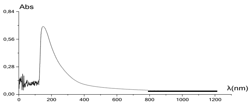
Figure 1: Spectrum of absorption of the aqua extract of Chamomile.
