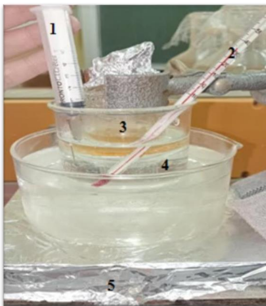
Figure II.19: system for drug release (1. Syringe for sampling, 2. Thermometer, 3. Membrane, 4. pH= 5.5, 5. Stirrer).
