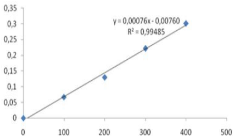
Figure 6: Flavonoid calibration curve.
