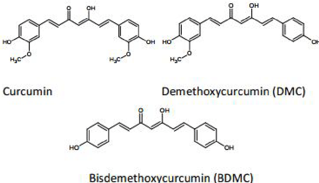
Figure I.10: Semi-developed structures of curcuminoids.
