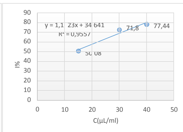
Figure III.24: Inhibition percentage of free radical DPPH in function of concentration of Thy extract.
