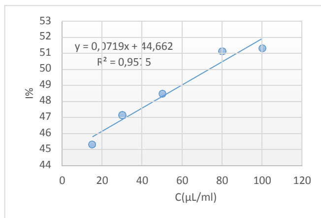
Figure III.23: Inhibition percentage of free radical DPPH in function of concentration of Cam extract.
