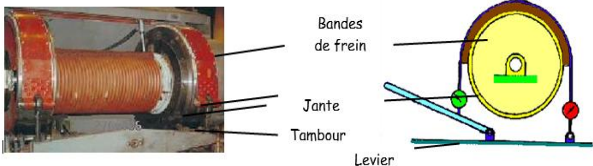
Figure I.5 : Le treuil
