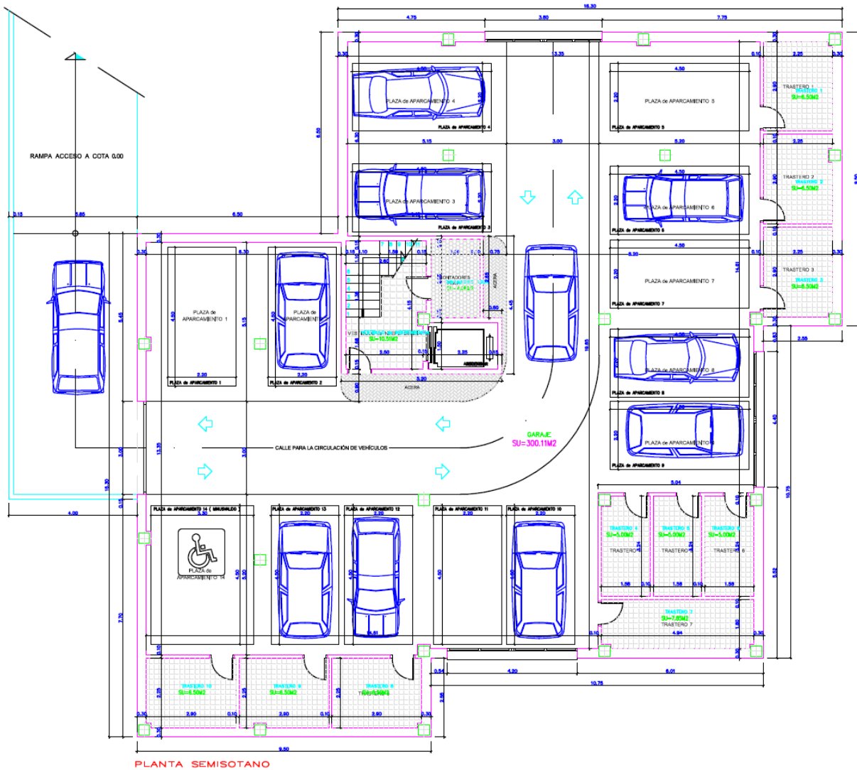
Figure I.1 : Plan R.D.C
