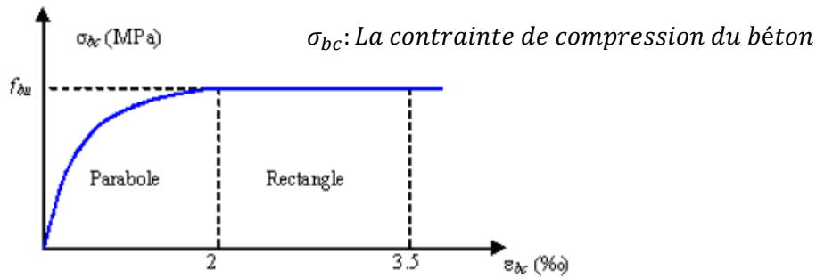
Figure I.1 : Diagramme parabolé – rectangle.
